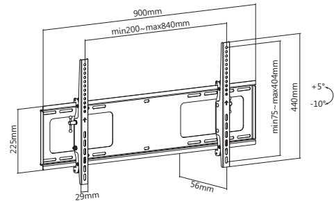
Dimensions (mm)
