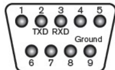
Male connector - 9 holes
